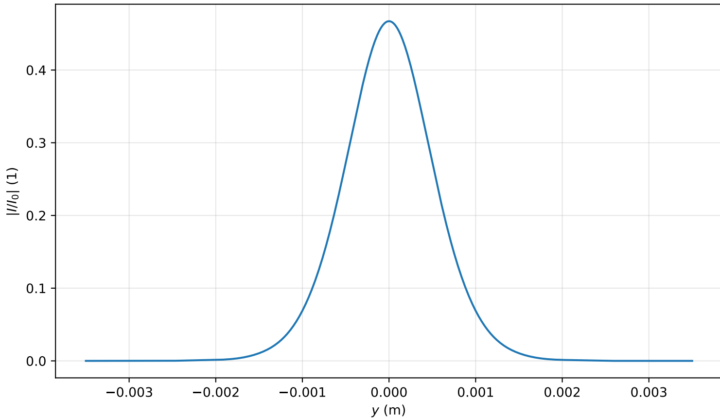
Intensity profile I(x=0, y, z=3.503)/I_0 , P_{in}=0.5P_{cr} , artificial time
